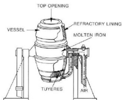
Gambar 2. 13 Tungku Converter Bessemer (Akuan, 2014)
