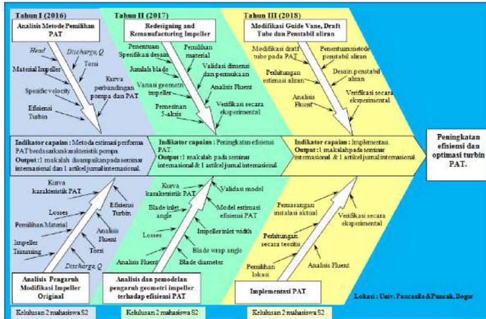
Gambar 3. 1 Bagan Penelitian
