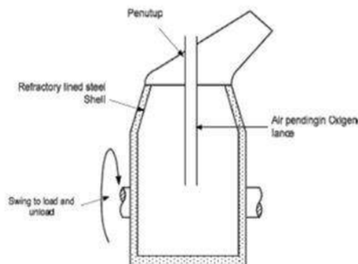
Gambar 2. 15 LD Top Blown Converter (Akuan, 2014)
