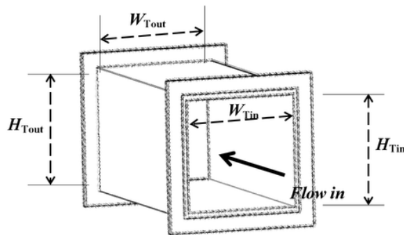
Gambar 2. 5. Test Section
