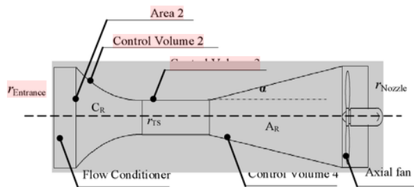
Gambar 2. 7. Terowongan Angin 2D
