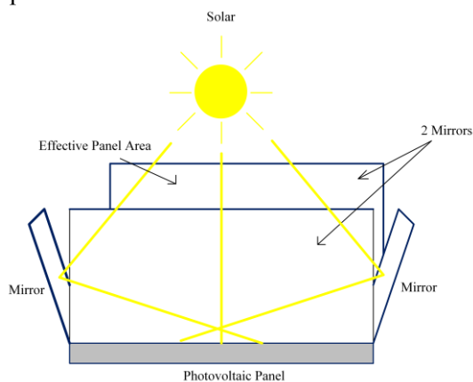
Fig. 1: PV module – 4 mirror systems
