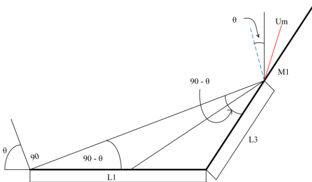
Fig. 5: The triangle geometry of the CPV system
