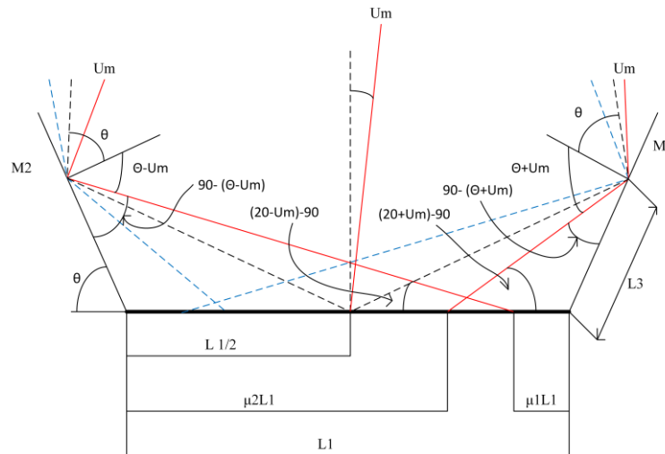
Fig. 4: The geometry model used for CPV systems
