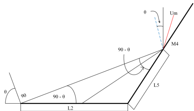
Fig. 6: The triangle geometry of the CPV system
