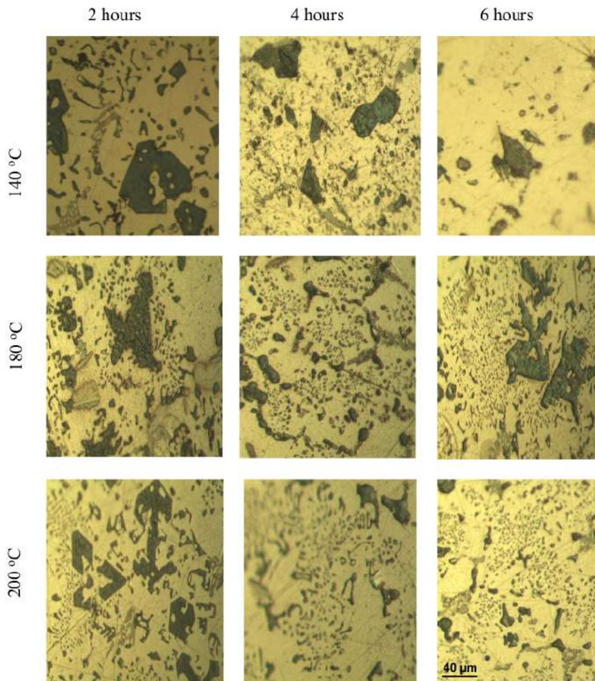
Fig. 3 Microstructure observations with 500x magnification on Al-7Si-Zn-Mg composite reinforced with SiC and Gr after aging at a temperature of 140 °C, 180 °C and 200 °C for 2, 4, and 6 hours.
