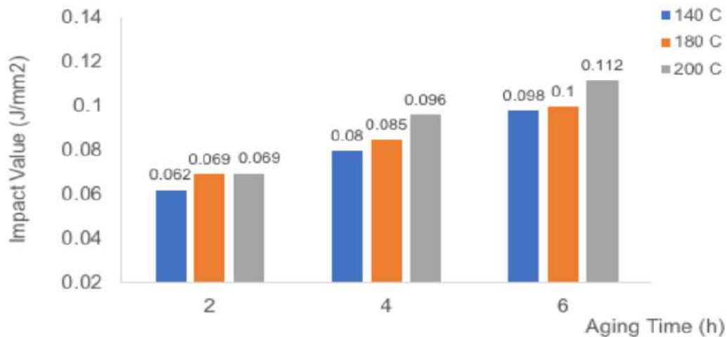
Fig. 2 Impact test of aluminum hybrid composite at the temperature of 140 °C, 180 °C and 200 °C with the holding time of 2, 4, and 6 hours.
