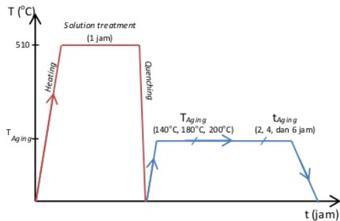
Gambar 6. Skema proses age hardening
